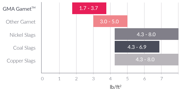
ABRASIVE CONSUMPTION
