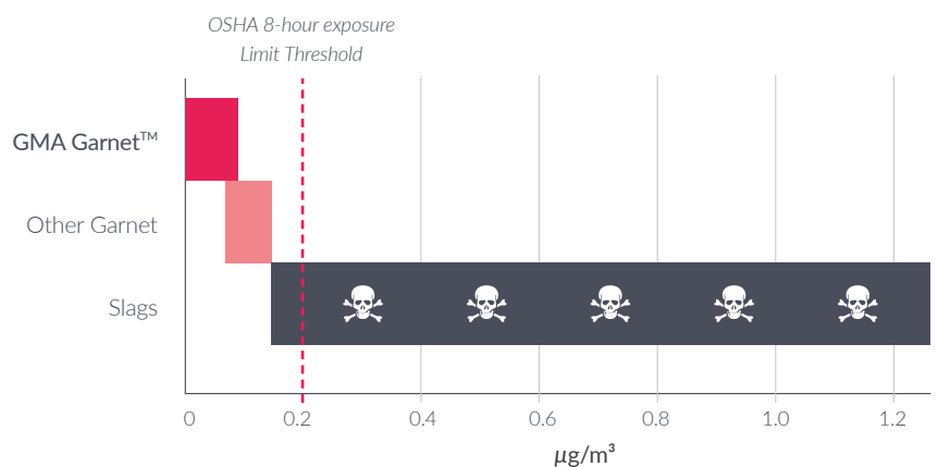
BERYLLIUM AIR SAMPLE - INDOOR (CONFINED SPACE, 8-HR TWA)
