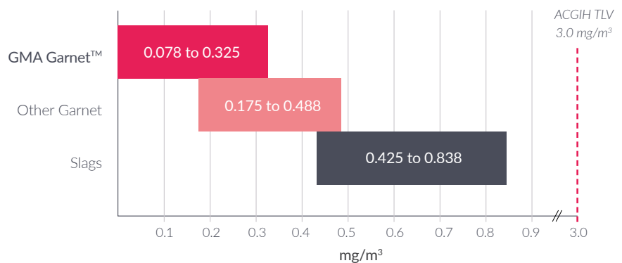
RESPIRABLE DUST AIR SAMPLE - OUTDOOR (20 FEET DOWNWIND, 8-HR TWA)
